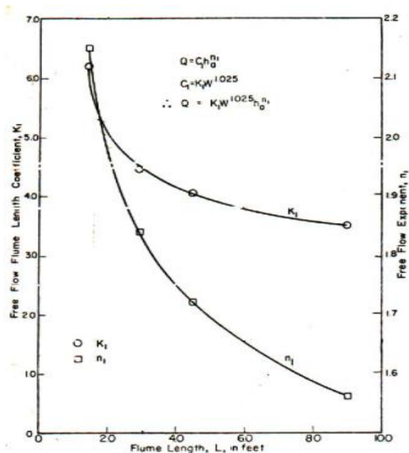
Figure 6: Generalized free flow ratings for Cutthroat flumes
