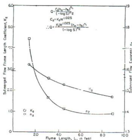
Figure 7: Generalized submerged flow ratings for Cutthroat flumes
